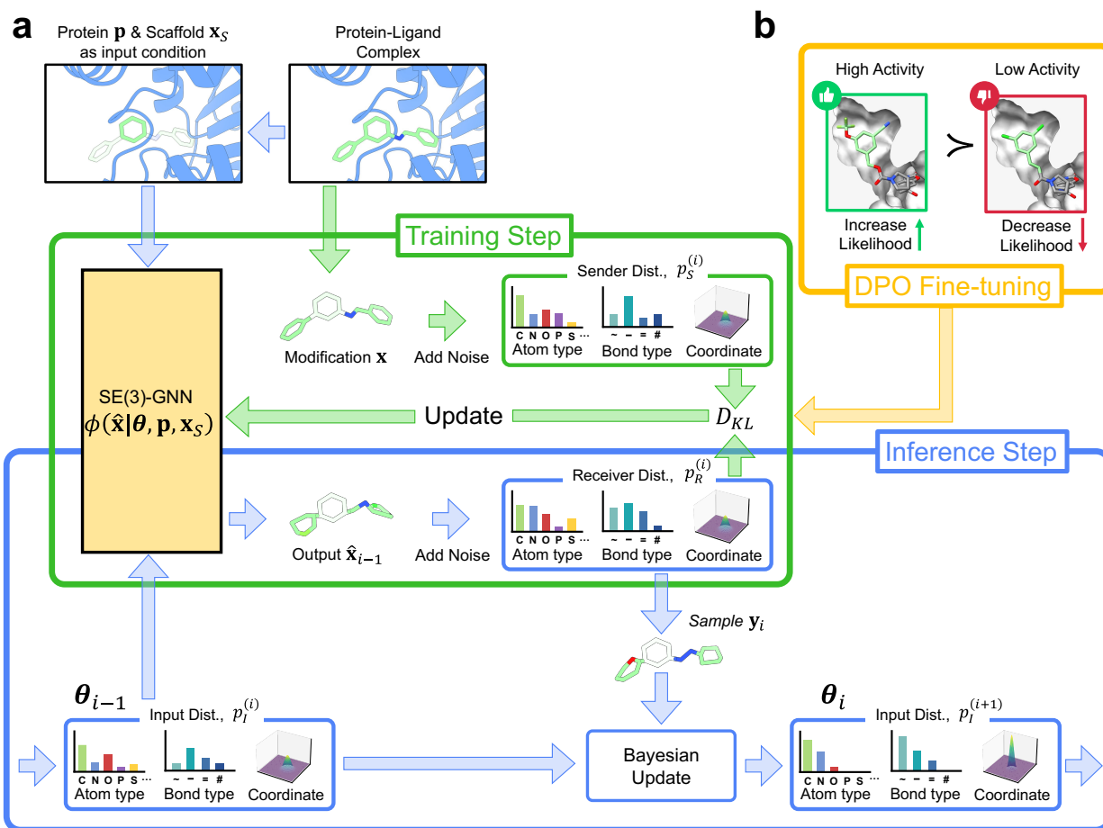
Fig. 2 An overview of the LeadFlow framework. a. The generative process of the LeadFlow for structure-based molecule optimization. It iteratively refines a set of parameters \boldsymbol{\theta} , using the SE(3)-equivariant graph transformer \phi to predict the clean modification \hat{\mathbf{x}}_{i-1} given current parameters \boldsymbol{\theta}_{i-1} with protein \mathbf{p} and scaffold conditions \mathbf{x}_S . The model is trained by minimizing the KL divergence between the sender distribution p_S over the noised observation \mathbf{y} of ground truth modification \mathbf{x} , and the receiver distribution p_R over the noised estimation \hat{\mathbf{y}} of predicted modification \hat{\mathbf{x}} . Through Bayesian update of the sampled \mathbf{y} , the parameters are iteratively refined from \boldsymbol{\theta}_{i-1} to \boldsymbol{\theta}_i , progressively enriching the information encoded in \boldsymbol{\theta} and enabling the model to predict increasingly accurate modifications \hat{\mathbf{x}} . LeadFlow uses the noise-reduced sampling strategy in which \hat{\mathbf{x}}_{i-1} is used in place of \mathbf{y}_i to directly perform the Bayesian update. b. DPO fine-tuning. Within each series, high-activity and low-activity modifications are paired for comparison, guiding the fine-tuning process to increase the likelihood of generating high-activity modifications.
